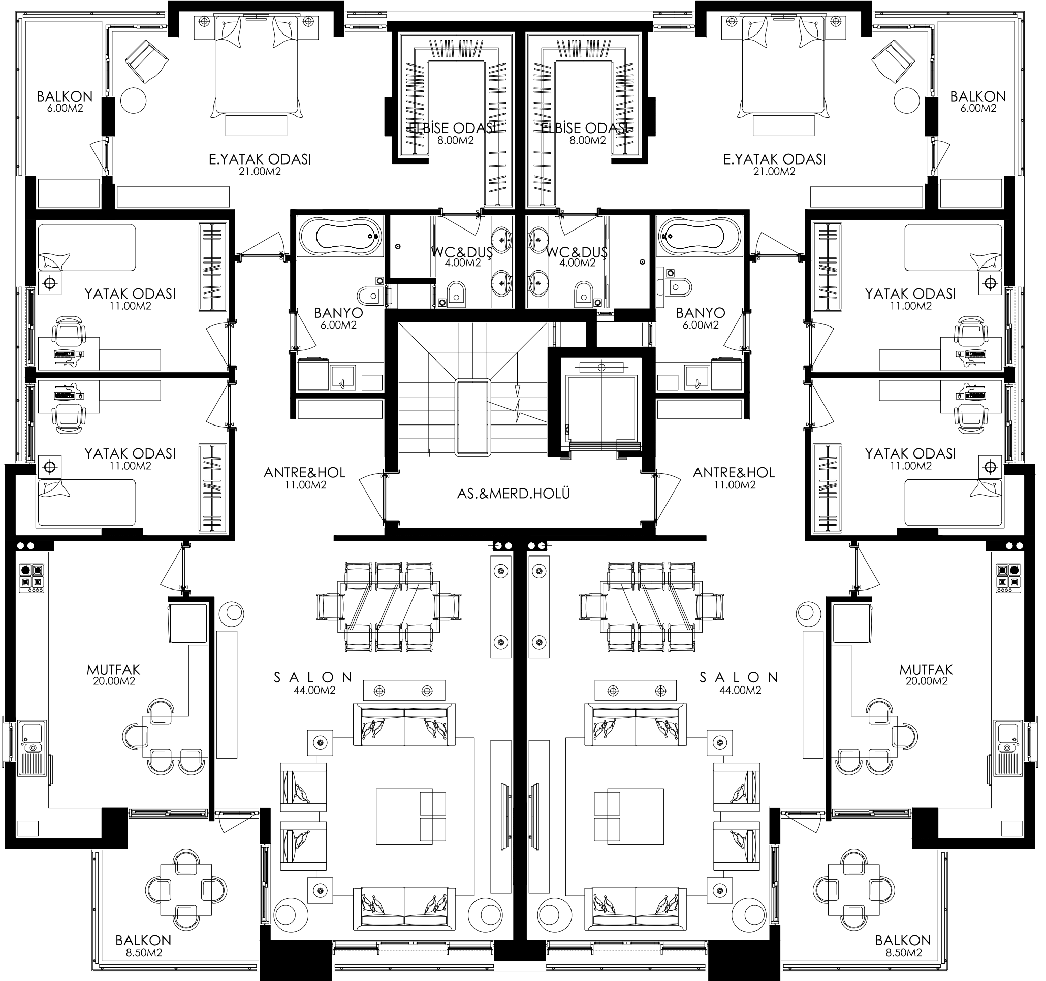
B-C-D-E-F BLOKLAR KAT PLANI
